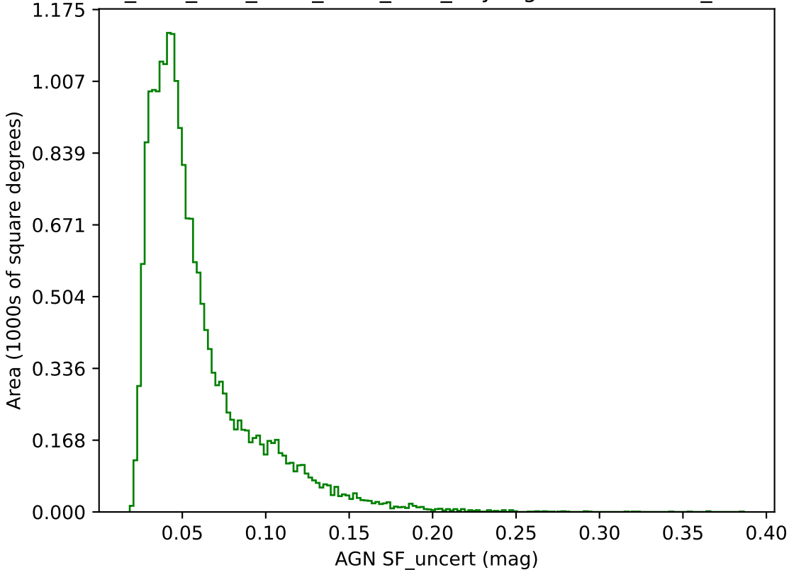
ddf_acor_sf25_lsf40_lsr10_v3.4_10yrs g band: AGN SF_uncert
