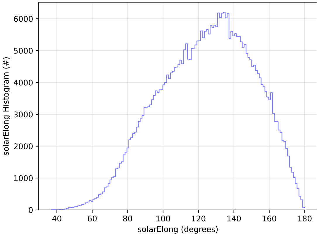
ddf_acor_sf25_lsf40_lsr10_v3.4_10yrs WFD y band: solarElong Histogram
