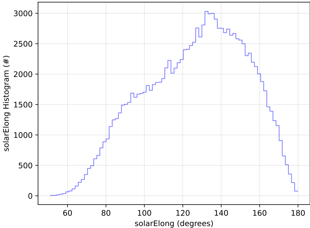
ddf_acor_sf25_lsf40_lsr10_v3.4_10yrs WFD u band: solarElong Histogram
