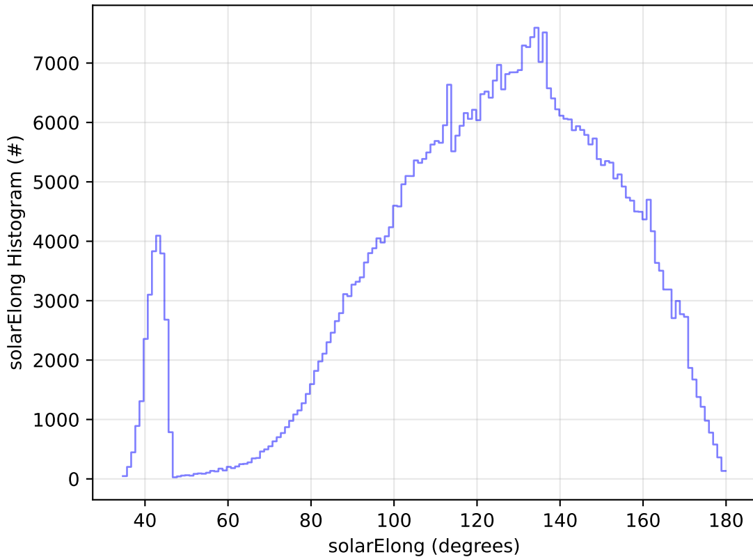
ddf_acor_sf25_lsf40_lsr10_v3.4_10yrs WFD i band: solarElong Histogram
