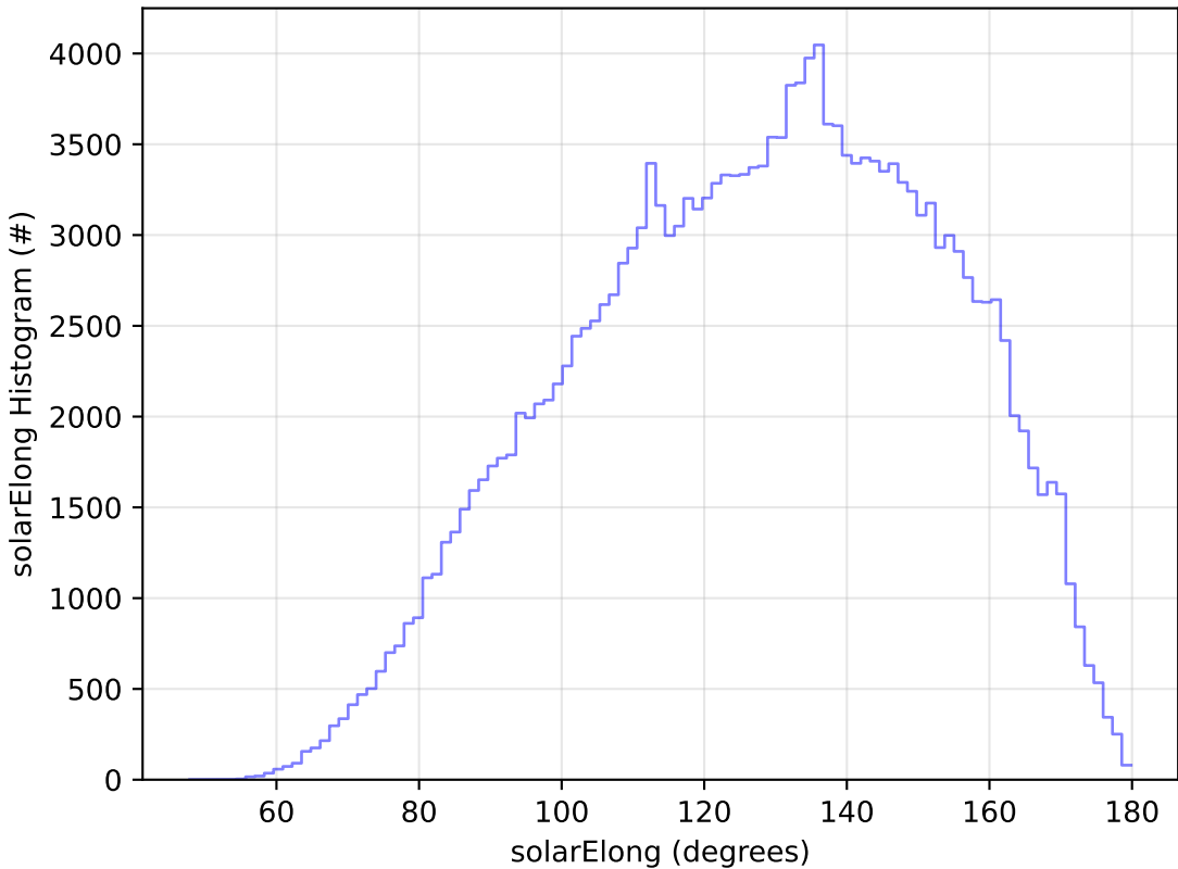
ddf_acor_sf25_lsf40_lsr10_v3.4_10yrs WFD g band: solarElong Histogram
