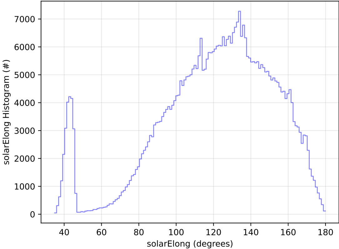
ddf_acor_sf25_lsf40_lsr10_v3.4_10yrs All sky z band: solarElong Histogram
