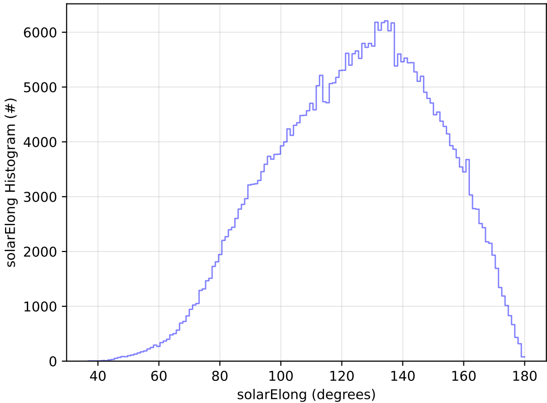
ddf_acor_sf25_lsf40_lsr10_v3.4_10yrs All sky y band: solarElong Histogram
