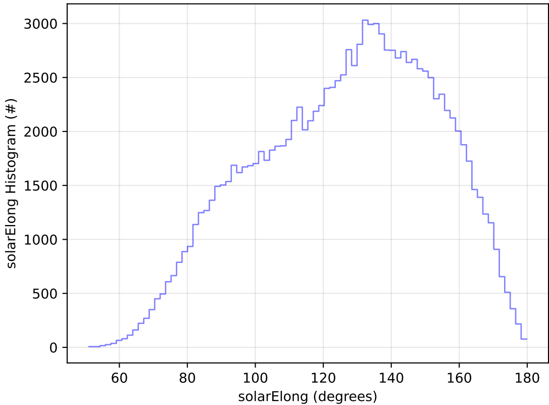
ddf_acor_sf25_lsf40_lsr10_v3.4_10yrs All sky u band: solarElong Histogram
