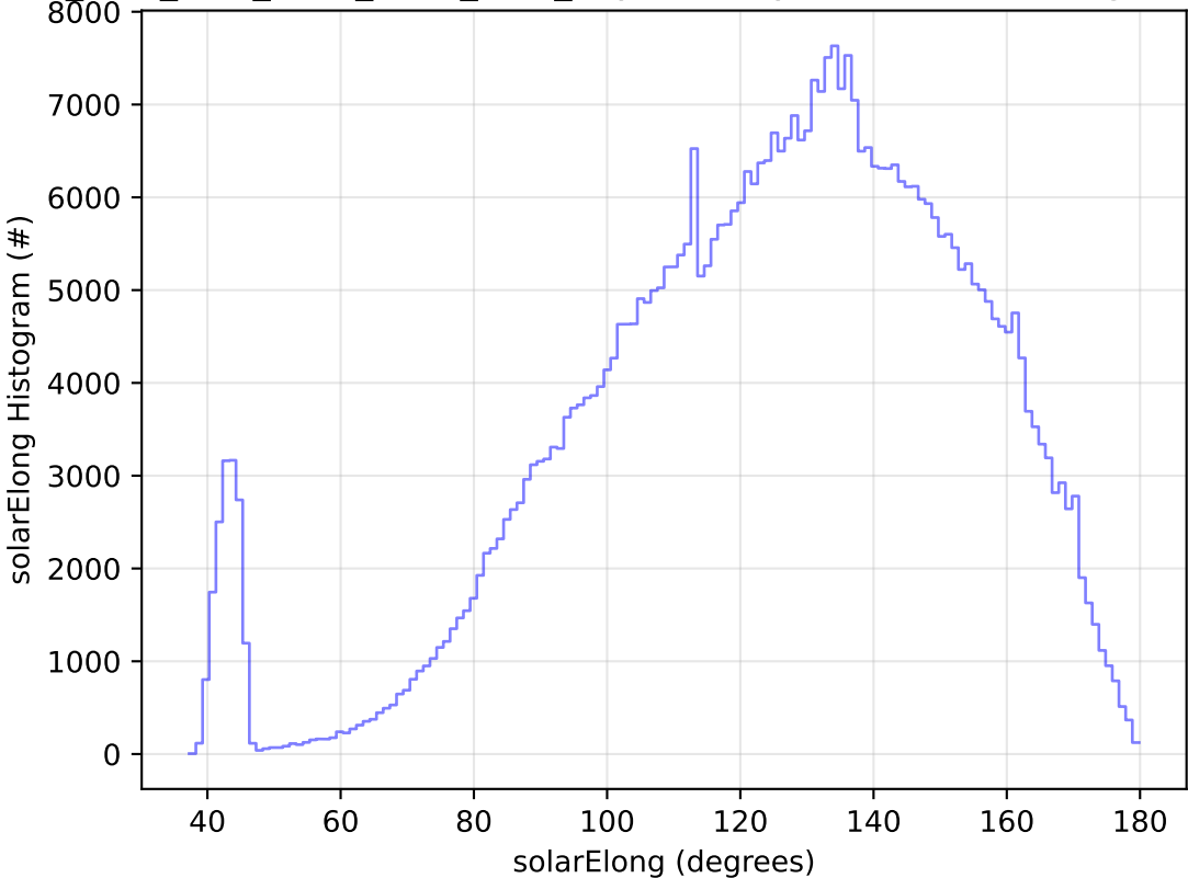
ddf_acor_sf25_lsf40_lsr10_v3.4_10yrs All sky r band: solarElong Histogram
