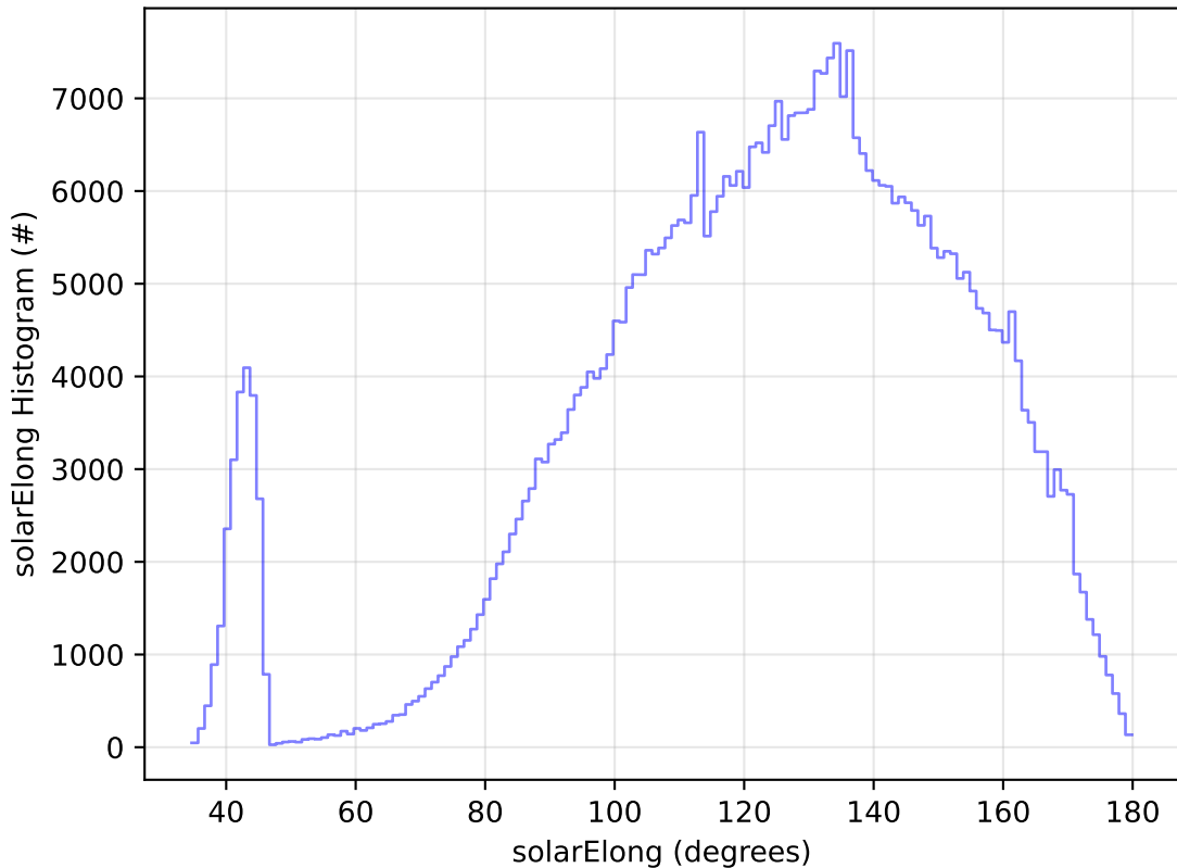
ddf_acor_sf25_lsf40_lsr10_v3.4_10yrs All sky i band: solarElong Histogram
