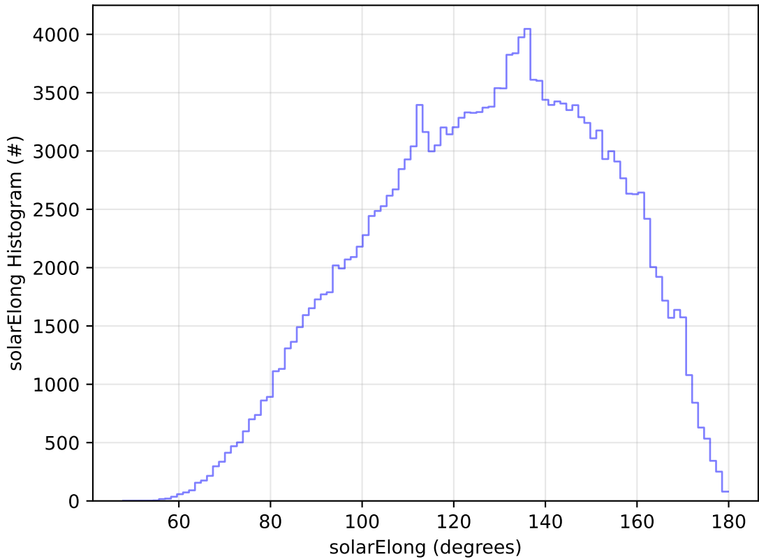
ddf_acor_sf25_lsf40_lsr10_v3.4_10yrs All sky g band: solarElong Histogram
