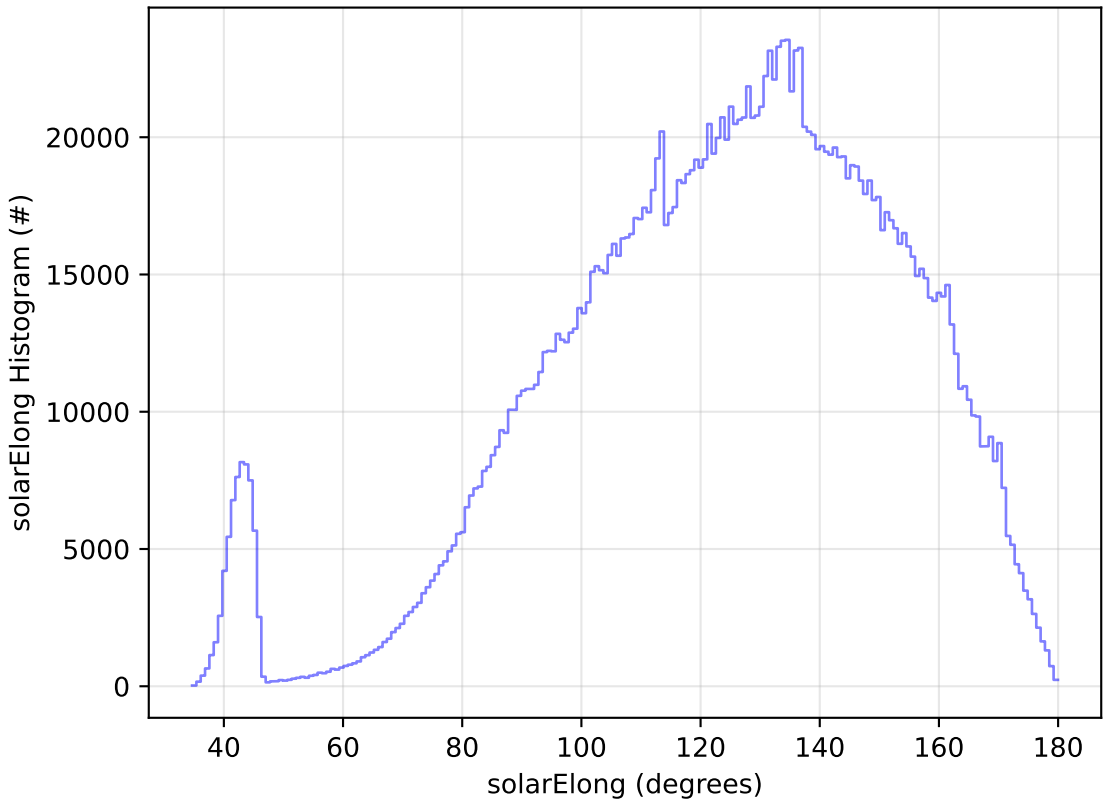
ddf_acor_sf25_lsf40_lsr10_v3.4_10yrs All sky all bands: solarElong Histogram
