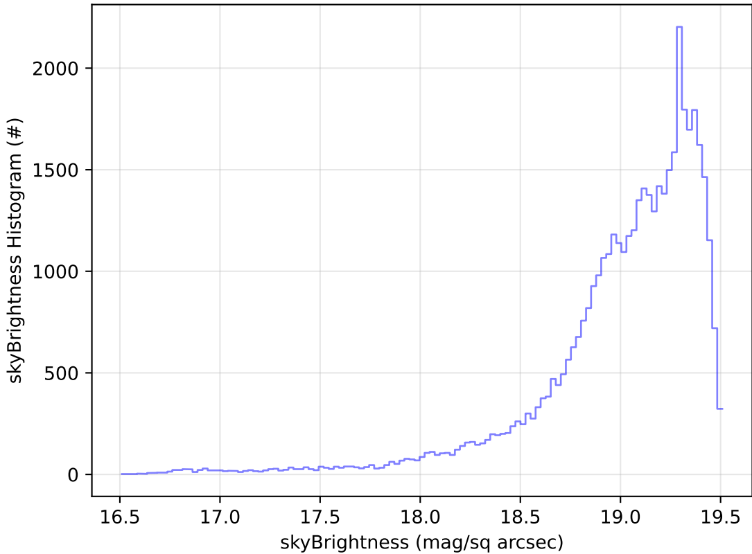
ddf_acor_sf25_lsf40_lsr10_v3.4_10yrs Yr 1 z band: skyBrightness Histogram
