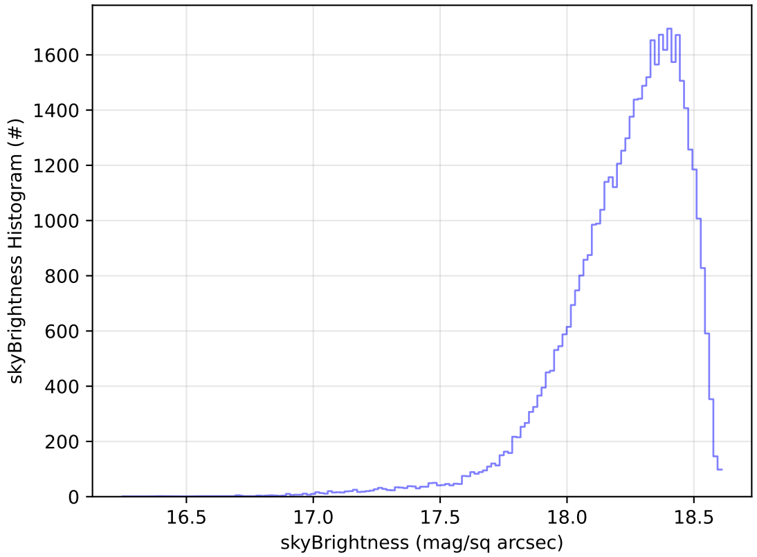
ddf_acor_sf25_lsf40_lsr10_v3.4_10yrs Yr 1 y band: skyBrightness Histogram
