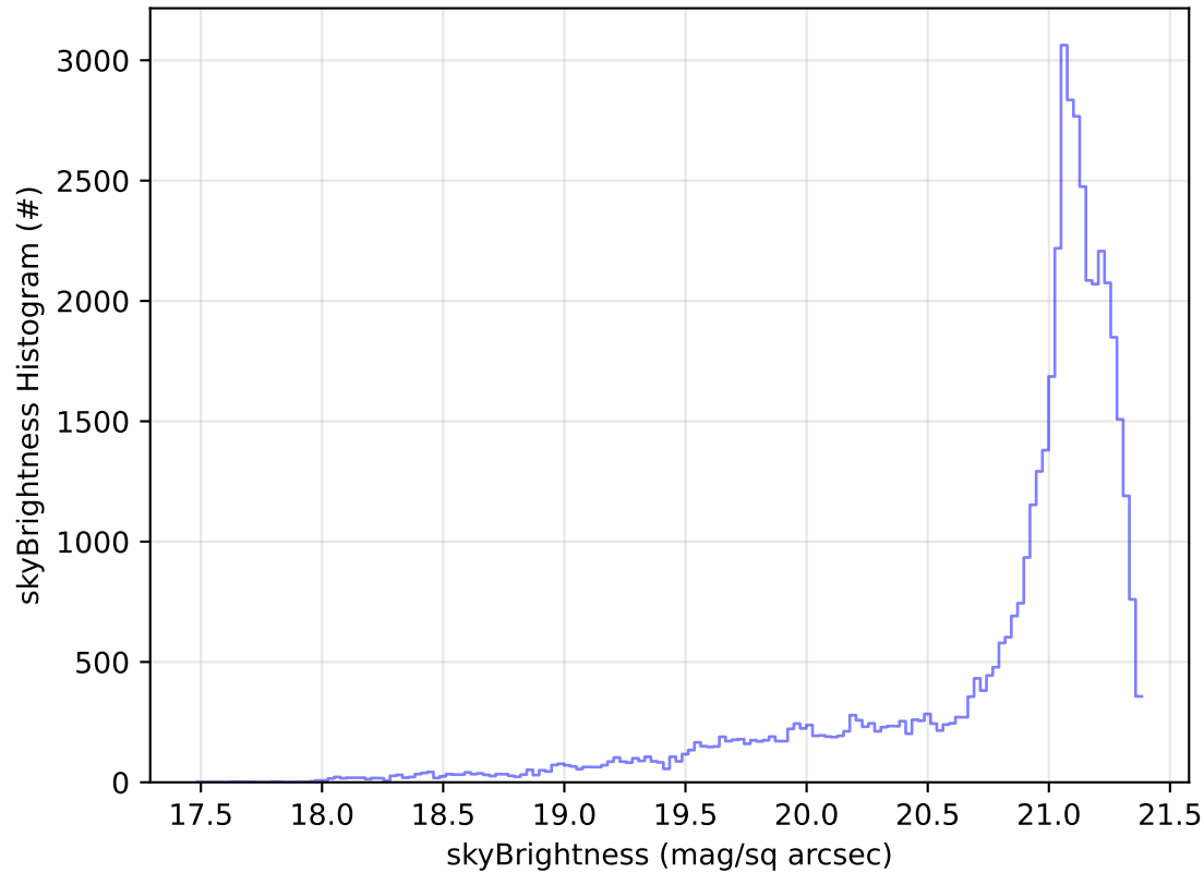
ddf_acor_sf25_lsf40_lsr10_v3.4_10yrs Yr 1 r band: skyBrightness Histogram
