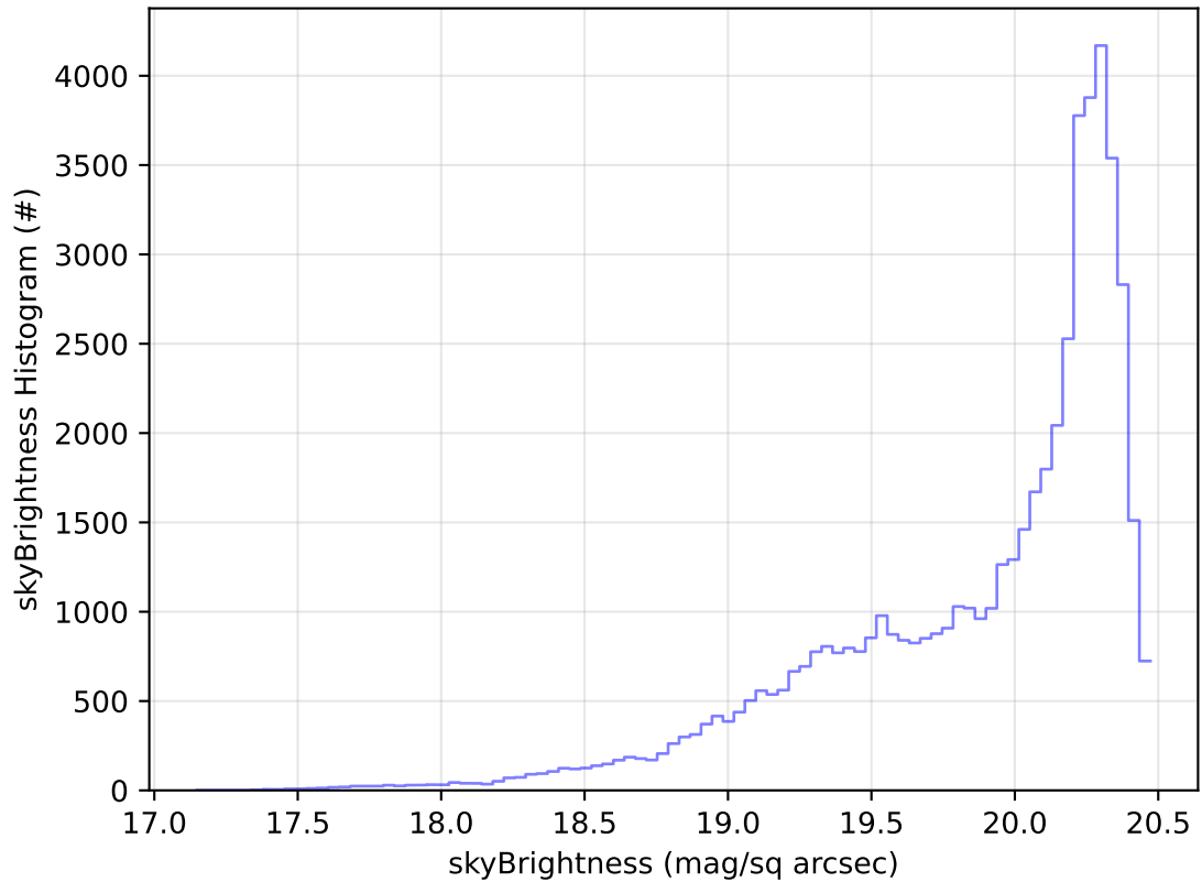
ddf_acor_sf25_lsf40_lsr10_v3.4_10yrs Yr 1 i band: skyBrightness Histogram
