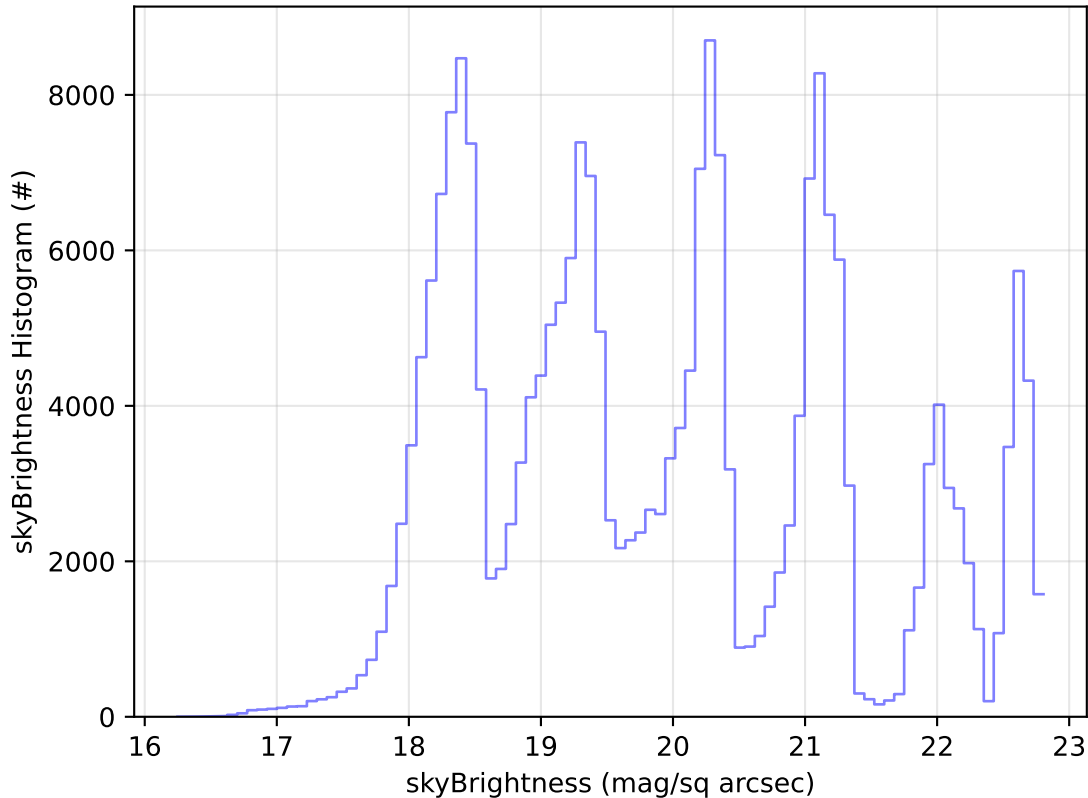
ddf_acor_sf25_lsf40_lsr10_v3.4_10yrs Yr 1 all bands: skyBrightness Histogram
