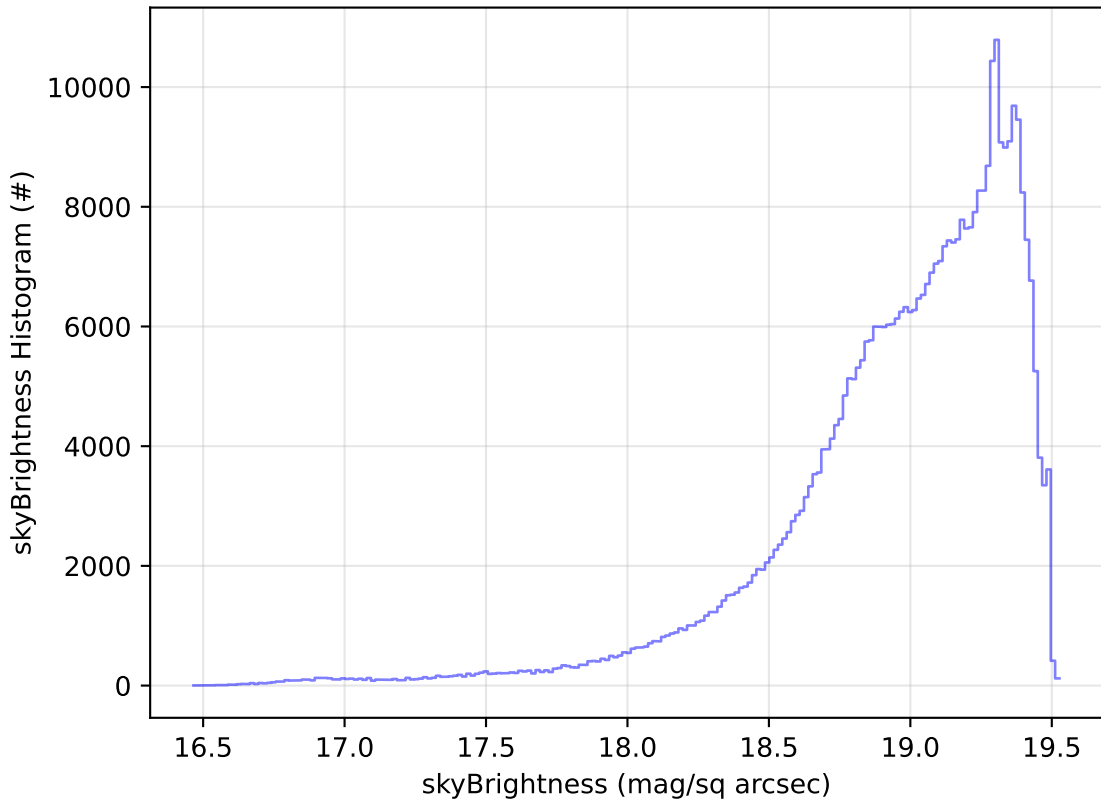
ddf_acor_sf25_lsf40_lsr10_v3.4_10yrs WFD z band: skyBrightness Histogram
