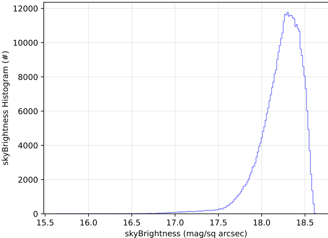
ddf_acor_sf25_lsf40_lsr10_v3.4_10yrs WFD y band: skyBrightness Histogram
