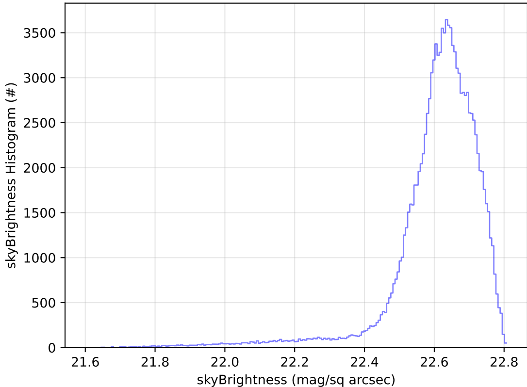
ddf_acor_sf25_lsf40_lsr10_v3.4_10yrs WFD u band: skyBrightness Histogram
