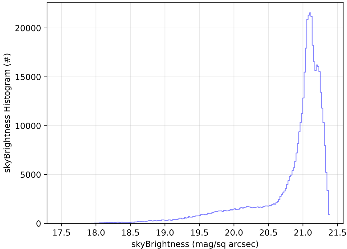
ddf_acor_sf25_lsf40_lsr10_v3.4_10yrs WFD r band: skyBrightness Histogram
