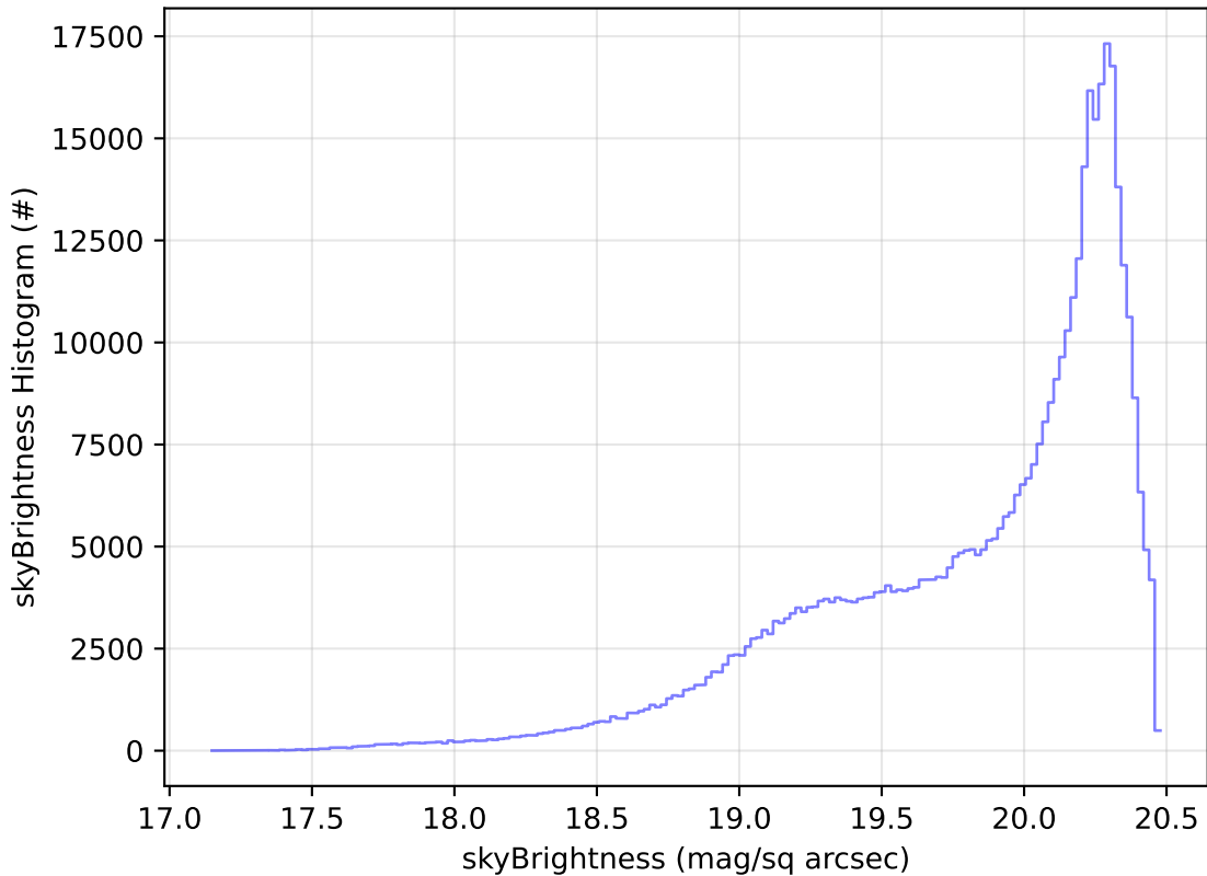
ddf_acor_sf25_lsf40_lsr10_v3.4_10yrs WFD i band: skyBrightness Histogram
