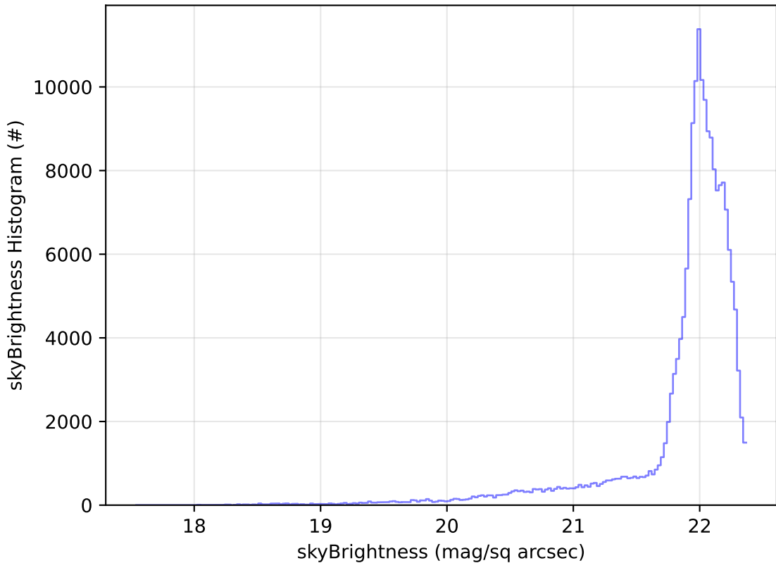
ddf_acor_sf25_lsf40_lsr10_v3.4_10yrs WFD g band: skyBrightness Histogram
