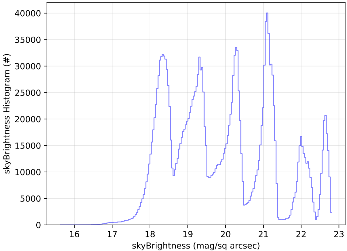
ddf_acor_sf25_lsf40_lsr10_v3.4_10yrs WFD all bands: skyBrightness Histogram
