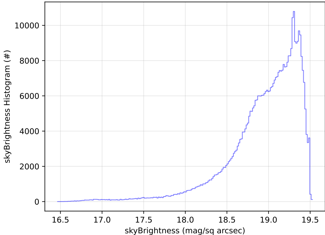
ddf_acor_sf25_lsf40_lsr10_v3.4_10yrs All sky z band: skyBrightness Histogram
