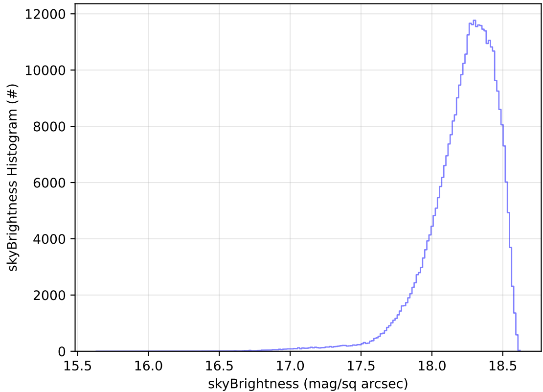
ddf_acor_sf25_lsf40_lsr10_v3.4_10yrs All sky y band: skyBrightness Histogram
