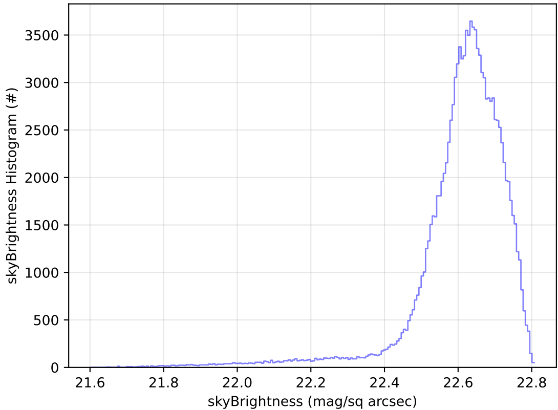
ddf_acor_sf25_lsf40_lsr10_v3.4_10yrs All sky u band: skyBrightness Histogram
