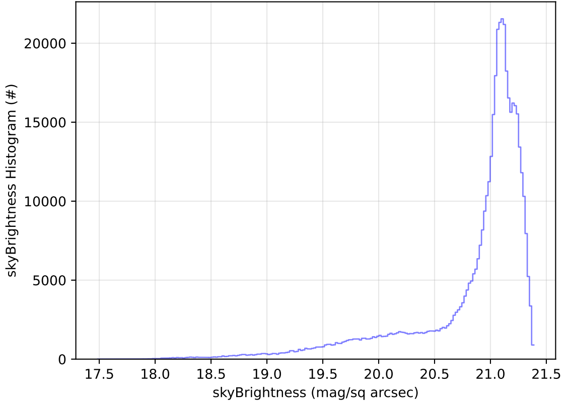
ddf_acor_sf25_lsf40_lsr10_v3.4_10yrs All sky r band: skyBrightness Histogram
