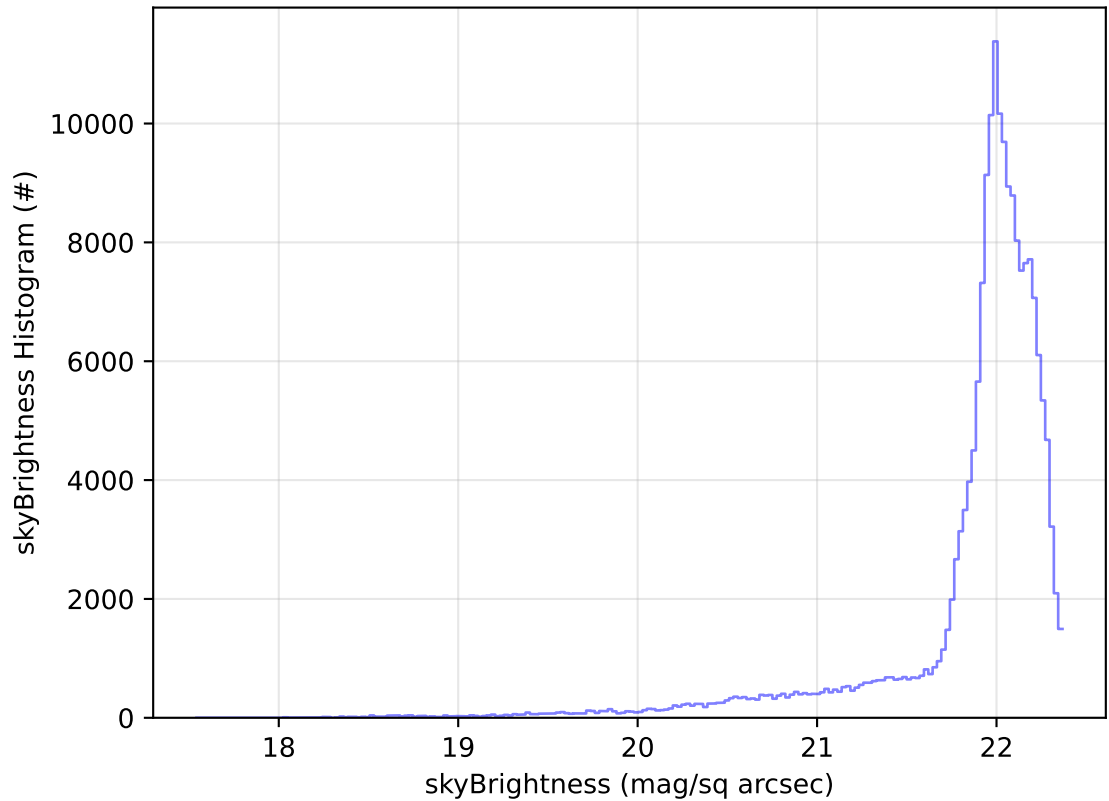
ddf_acor_sf25_lsf40_lsr10_v3.4_10yrs All sky g band: skyBrightness Histogram
