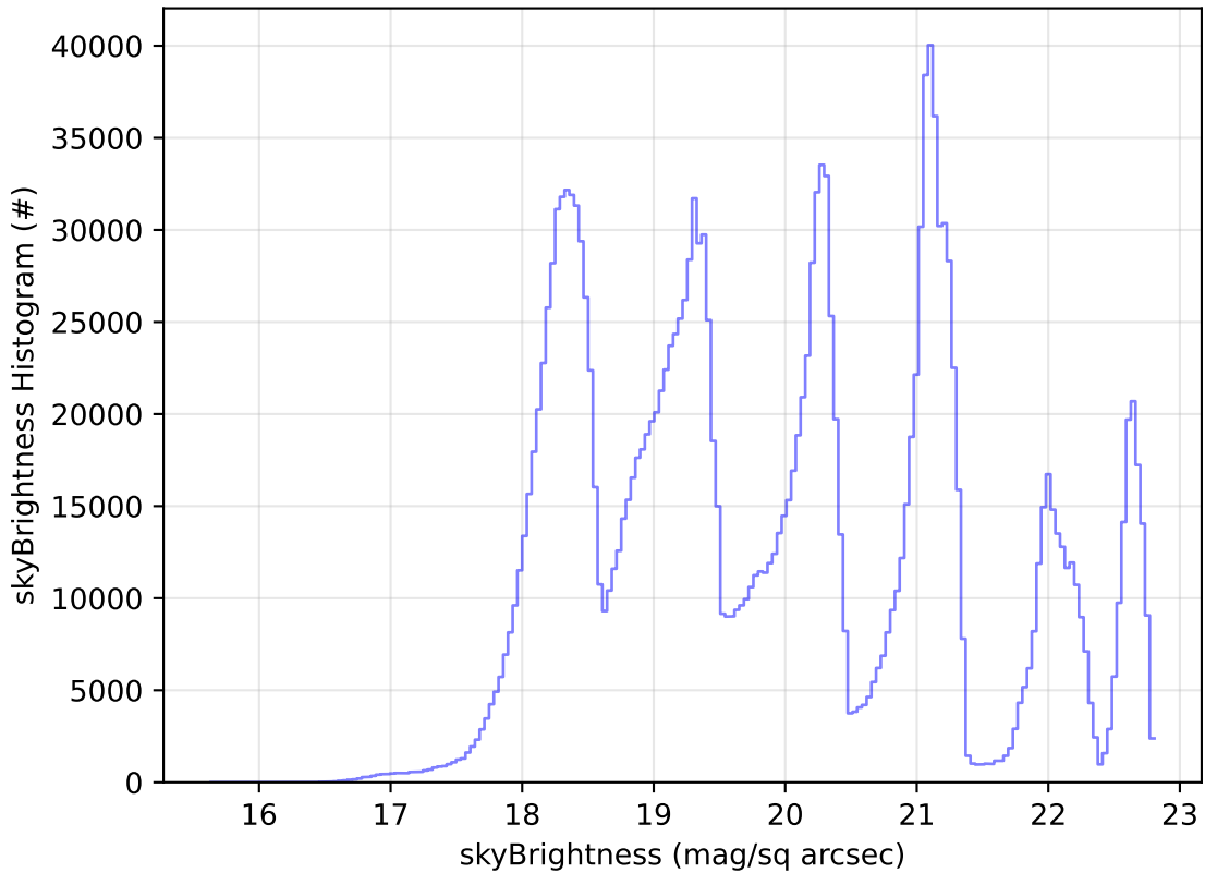
ddf_acor_sf25_lsf40_lsr10_v3.4_10yrs All sky all bands: skyBrightness Histogram
