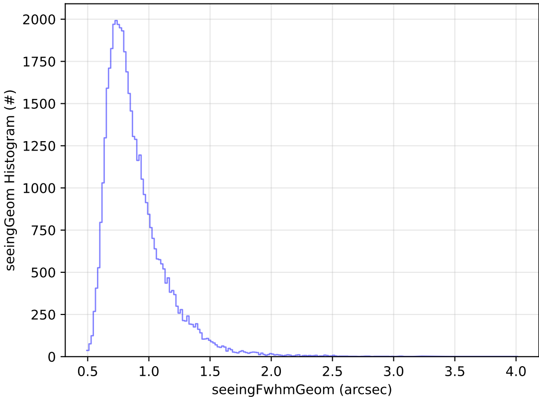
ddf_acor_sf25_lsf40_lsr10_v3.4_10yrs Yr 1 z band: seeingGeom Histogram
