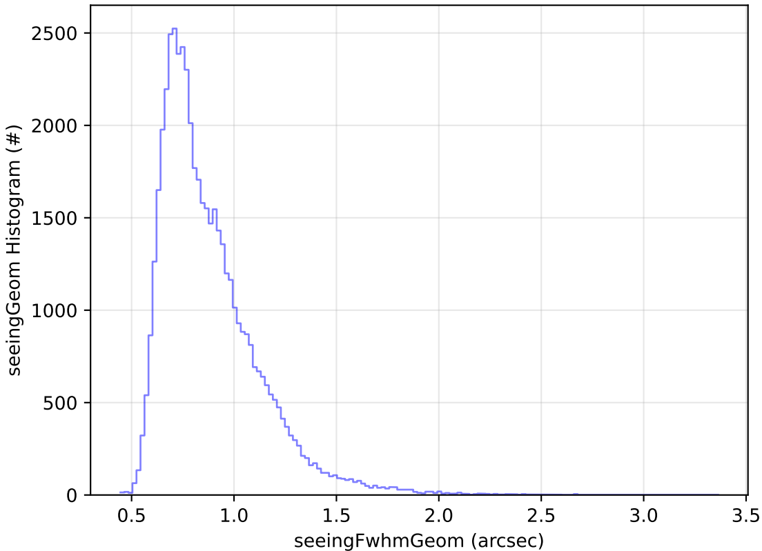
ddf_acor_sf25_lsf40_lsr10_v3.4_10yrs Yr 1 r band: seeingGeom Histogram
