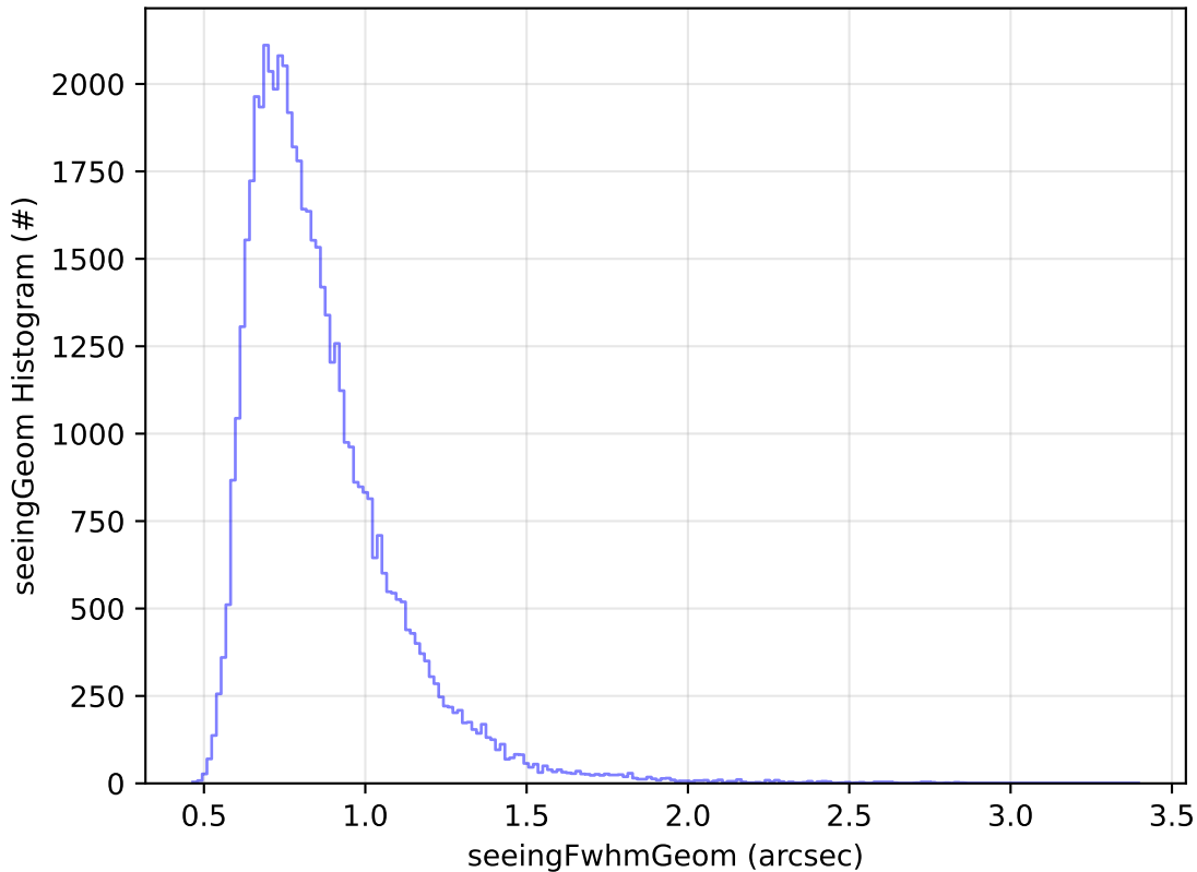
ddf_acor_sf25_lsf40_lsr10_v3.4_10yrs Yr 1 i band: seeingGeom Histogram
