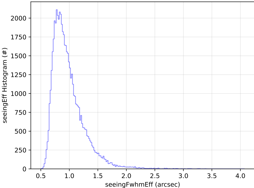
ddf_acor_sf25_lsf40_lsr10_v3.4_10yrs Yr 1 i band: seeingEff Histogram
