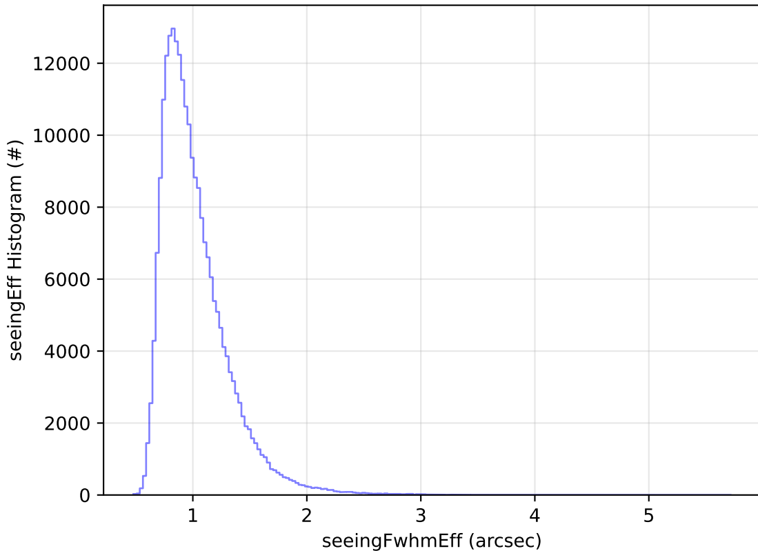
ddf_acor_sf25_Isf40_Isr10_v3.4_10yrs Yr 1 all bands: seeingEff Histogram
