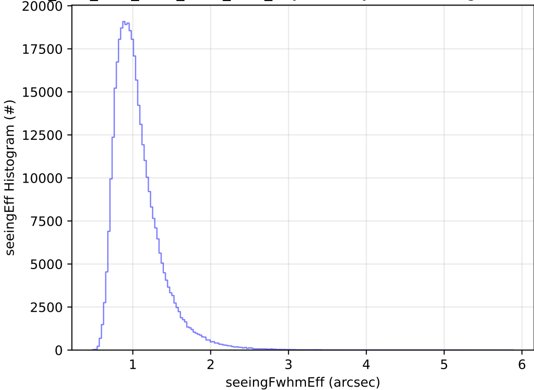
ddf_acor_sf25_lsf40_lsr10_v3.4_10yrs WFD y band: seeingEff Histogram
