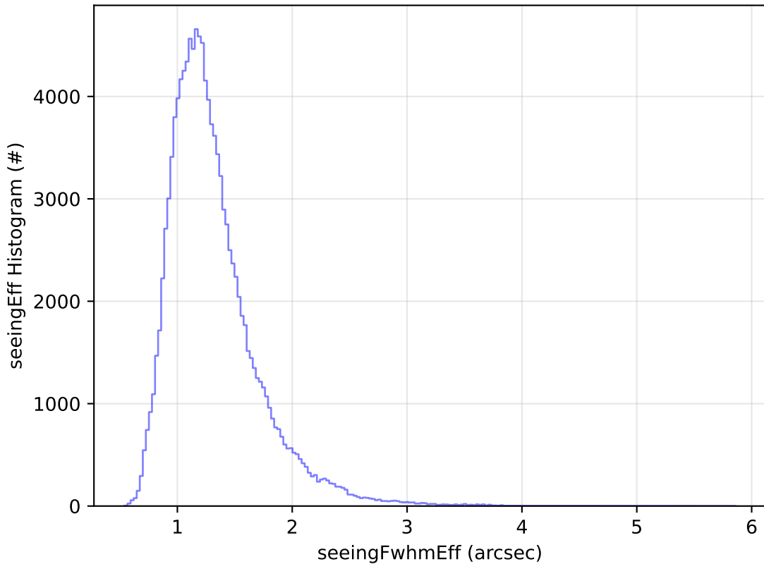
ddf_acor_sf25_lsf40_lsr10_v3.4_10yrs WFD u band: seeingEff Histogram
