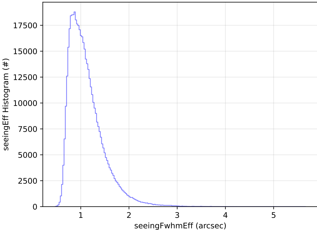
ddf_acor_sf25_lsf40_lsr10_v3.4_10yrs WFD r band: seeingEff Histogram
