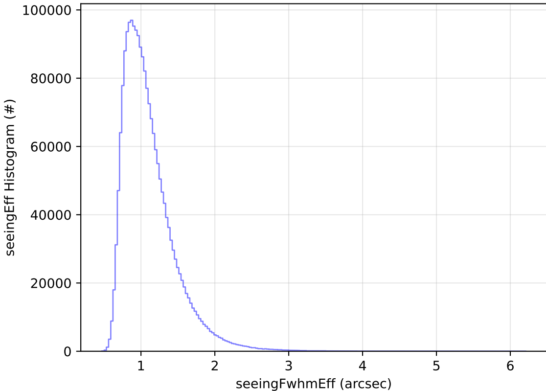
ddf_acor_sf25_lsf40_lsr10_v3.4_10yrs WFD all bands: seeingEff Histogram
