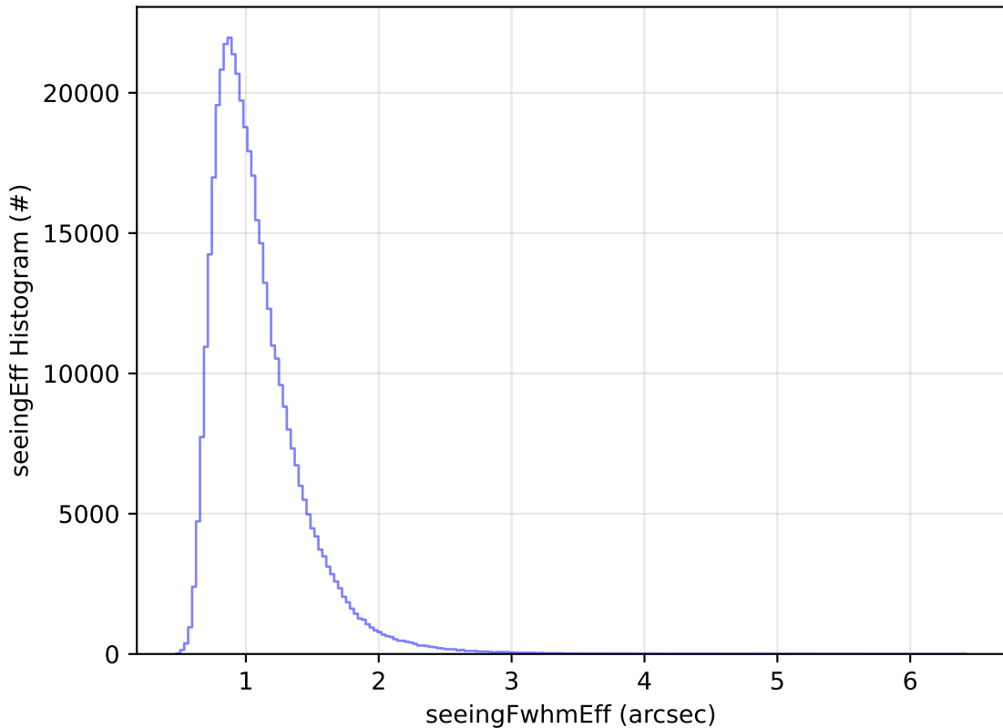
ddf_acor_sf25_Isf40_Isr10_v3.4_10yrs All sky z band: seeingEff Histogram
