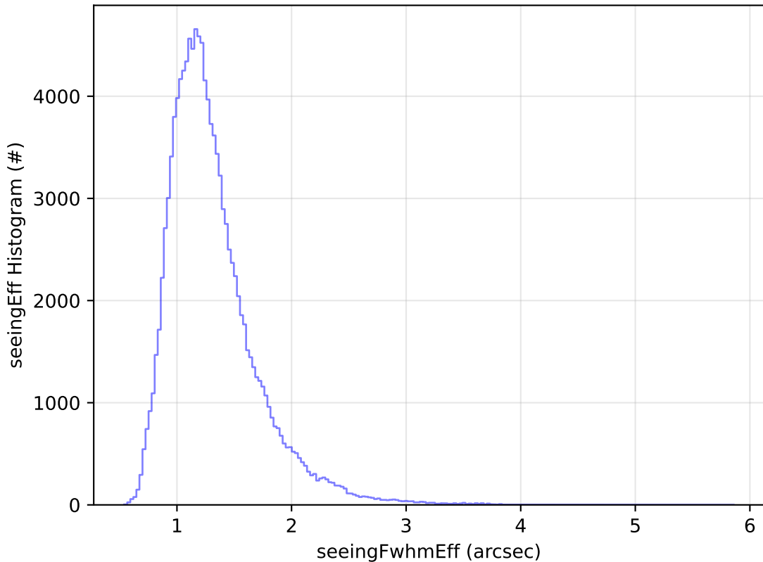
ddf_acor_sf25_ls40_lsr10_v3.4_10yrs All sky u band: seeingEff Histogram
