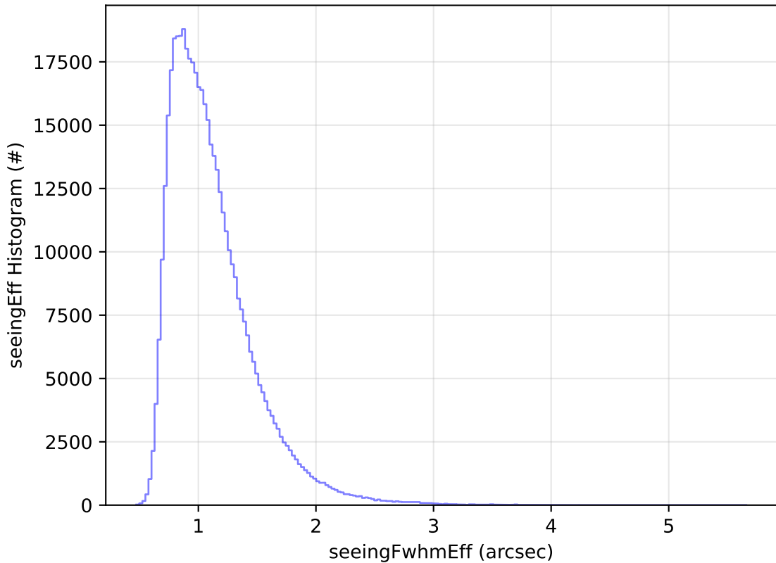
ddf_acor_sf25_lsf40_lsr10_v3.4_10yrs All sky r band: seeingEff Histogram
