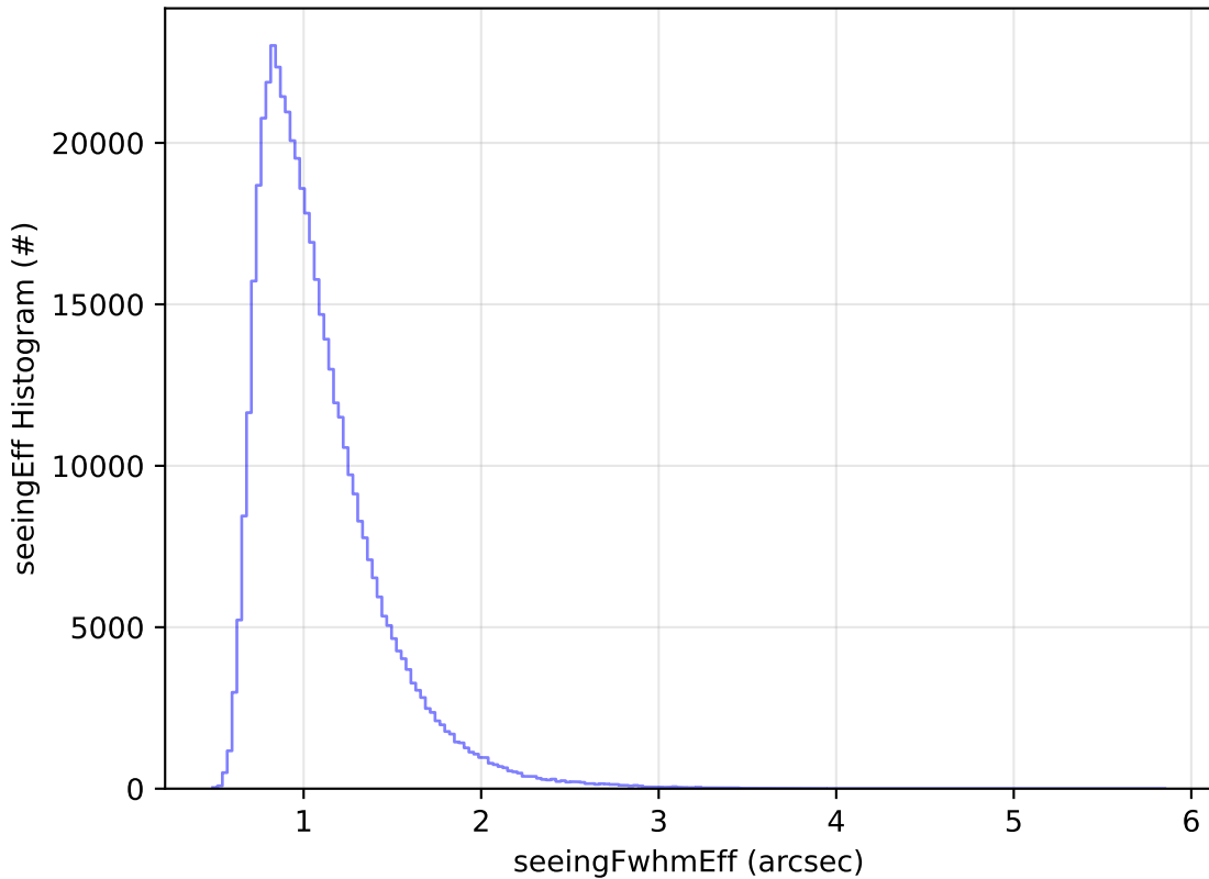
ddf_acor_sf25_lsf40_lsr10_v3.4_10yrs All sky i band: seeingEff Histogram
