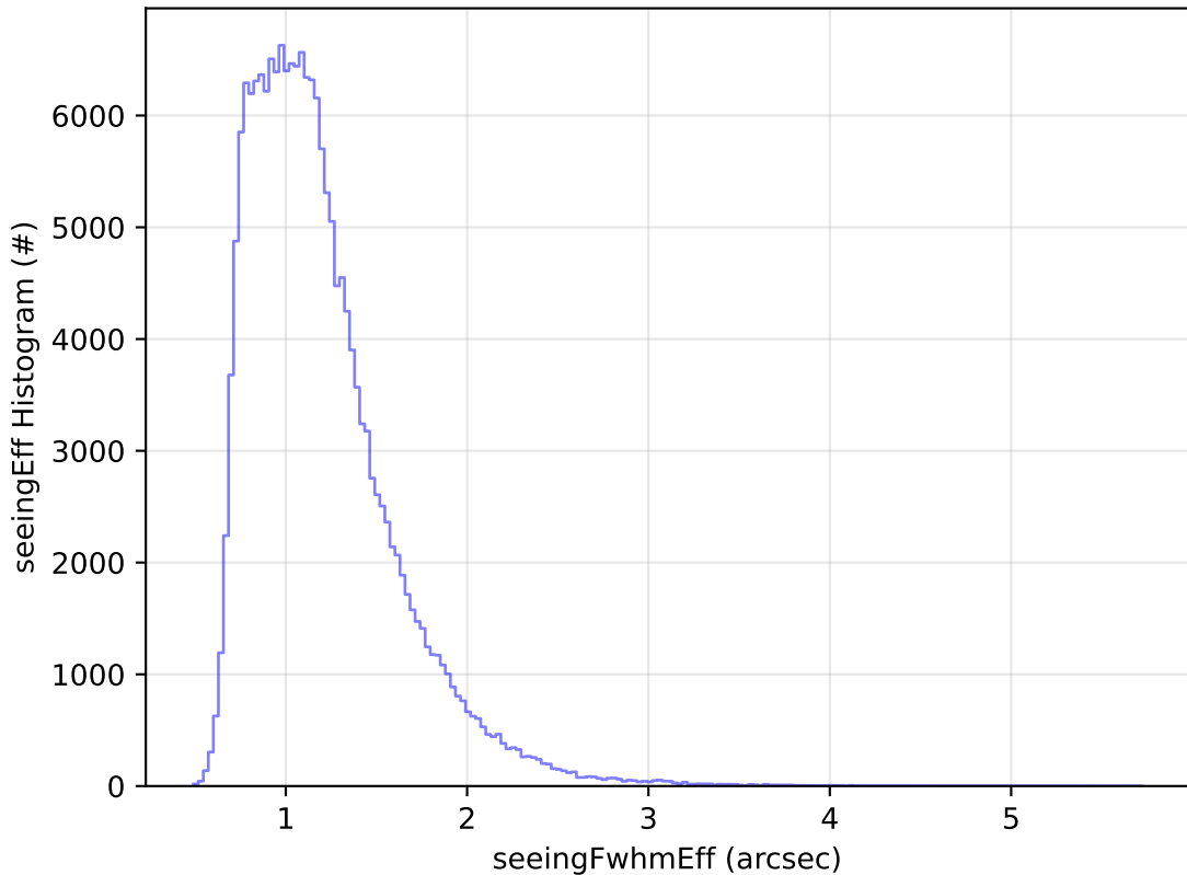
ddf_acor_sf25_ls40_lsr10_v3.4_10yrs All sky g band: seeingEff Histogram
