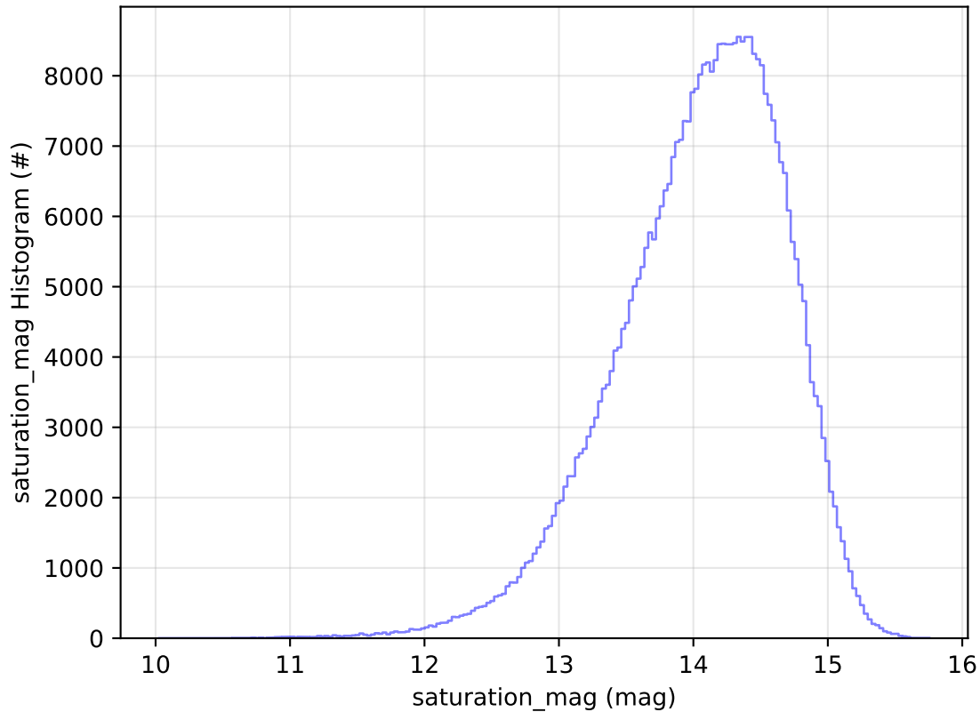
ddf_acor_sf25_lsf40_lsr10_v3.4_10yrs WFD z band: saturation_mag Histogram
