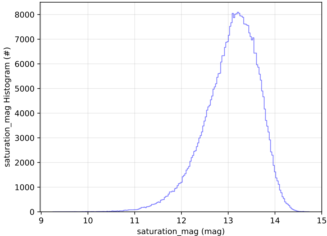
ddf_acor_sf25_lsf40_lsr10_v3.4_10yrs WFD y band: saturation_mag Histogram
