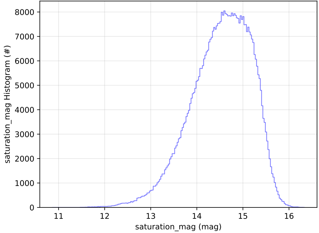
ddf_acor_sf25_lsf40_lsr10_v3.4_10yrs WFD r band: saturation_mag Histogram
