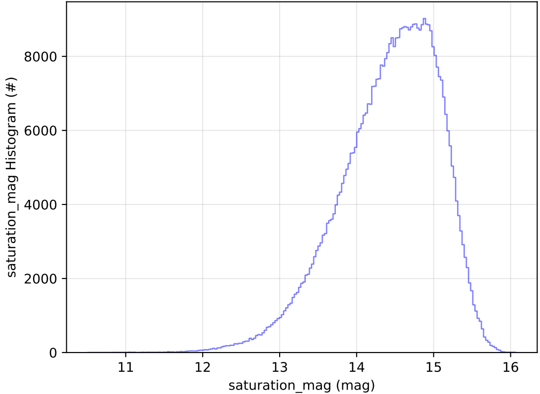
ddf_acor_sf25_lsf40_lsr10_v3.4_10yrs WFD i band: saturation_mag Histogram
