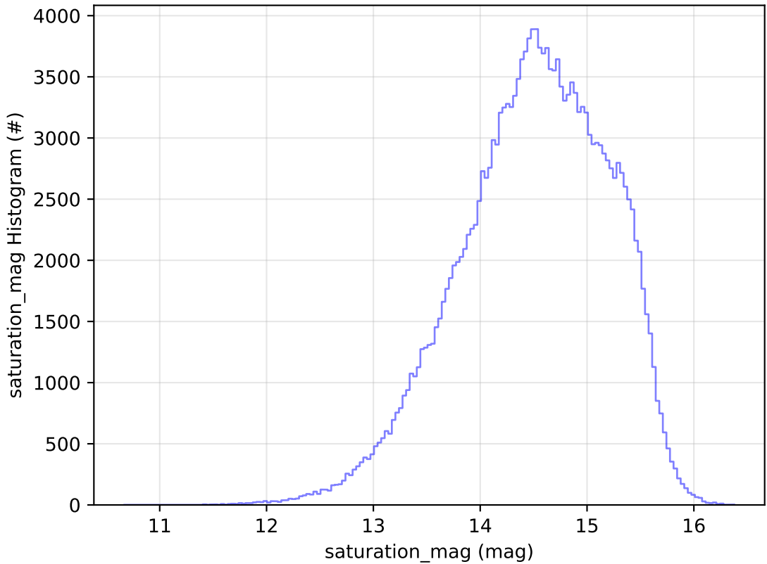
ddf_acor_sf25_lsf40_lsr10_v3.4_10yrs WFD g band: saturation_mag Histogram
