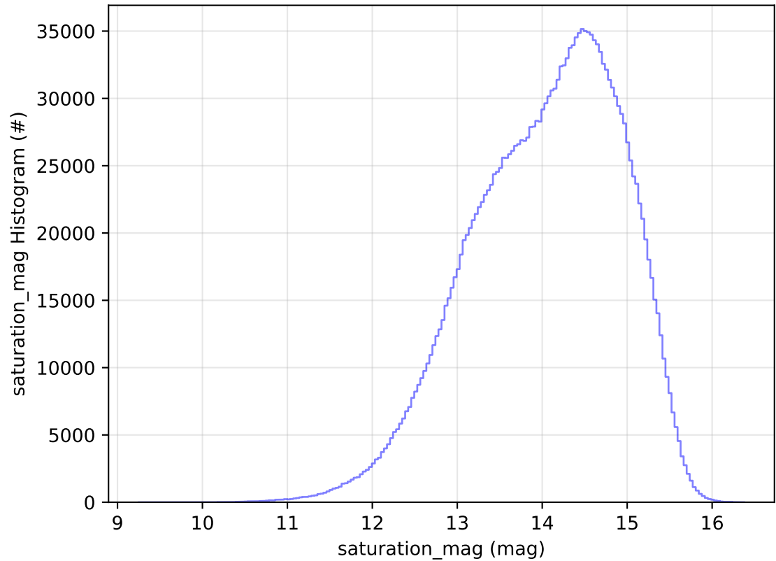
ddf_acor_sf25_lsf40_lsr10_v3.4_10yrs WFD all bands: saturation_mag Histogram
